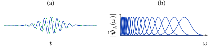
Fig. 2: (a) Real and imaginary parts of a Morlet mother wavelet with Q = 4 . (b) The wavelet filters in the frequency domain.
