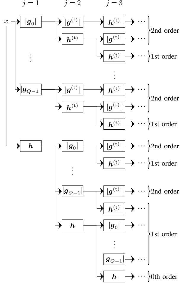
Fig. 5: A time scattering network. Each block with |g_k| or |g^{(t)}| outputs the modulus of the input convolved with a band-pass filter, subsampled by 2. Blocks with h and h^{(t)} convolves the input with a low-pass filter and subsample by 2.
